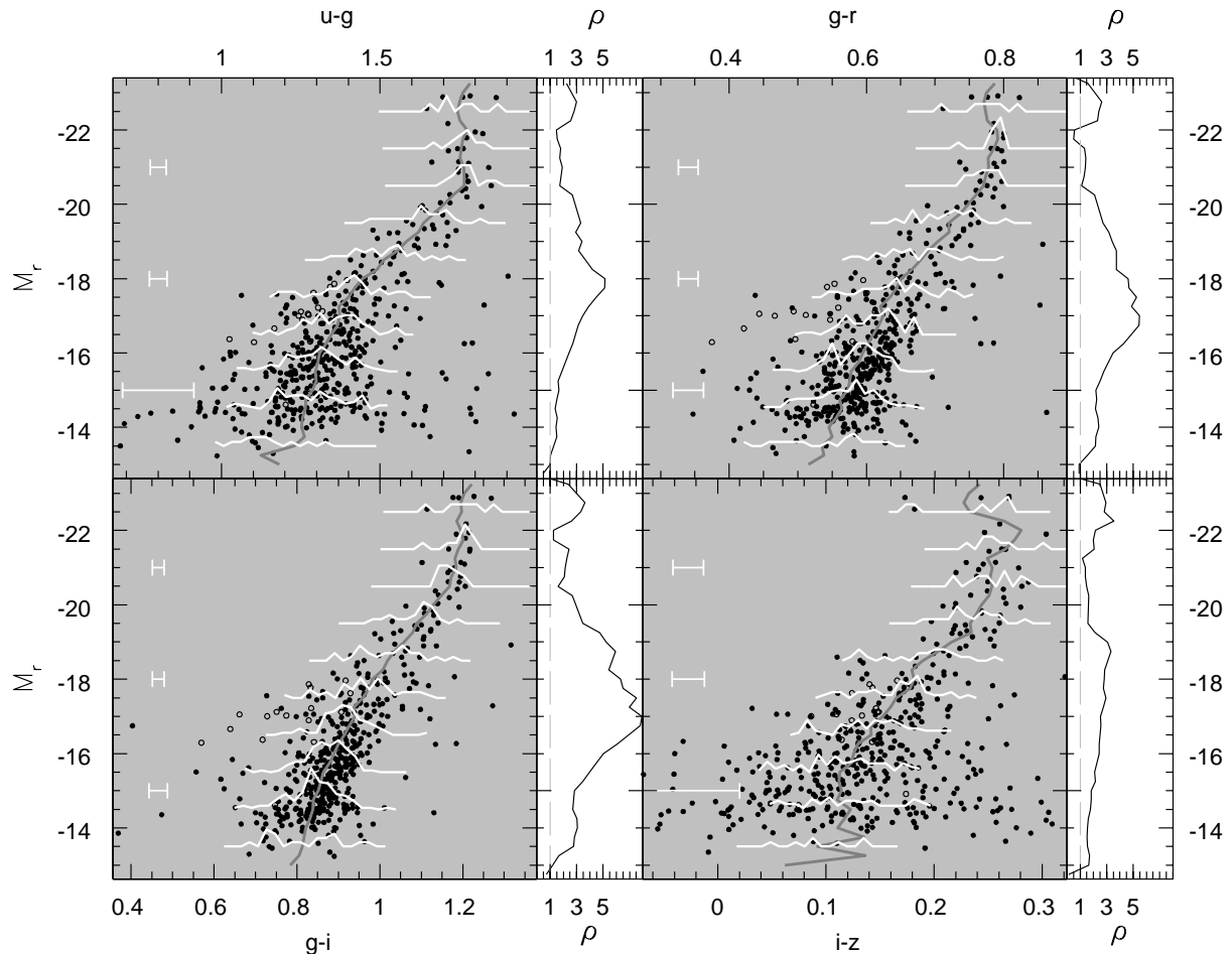
FIG. 1.— Color Magnitude Relations for the colors u - g , g - r , g - i , and i - z . Open circles show dEs with blue cores and filled circles all the other galaxies in the sample. Limits for the x-axes are scaled to the mean color of galaxies fainter than M_r > -15 mag and brighter than M_r < -21 mag. The gray line indicates the “running histogram” as found in successive magnitude bins with a width of 1 mag and steps of 0.25 mag, clipped one time at 3\sigma . We limit the drawing range for the line to the region with at least three galaxies in a bin. The white histograms show the distributions in bins of the same width, normalized to the square root of the number of galaxies in the bin, shown for every fourth step. The white errorbars indicate typical photometric errors at the respective brightness. In the panels right to the color magnitude diagrams a measure for the intrinsic scatter is given by the ratio of the RMS of the scatter and of the photometric error in the same running bins (see text).
