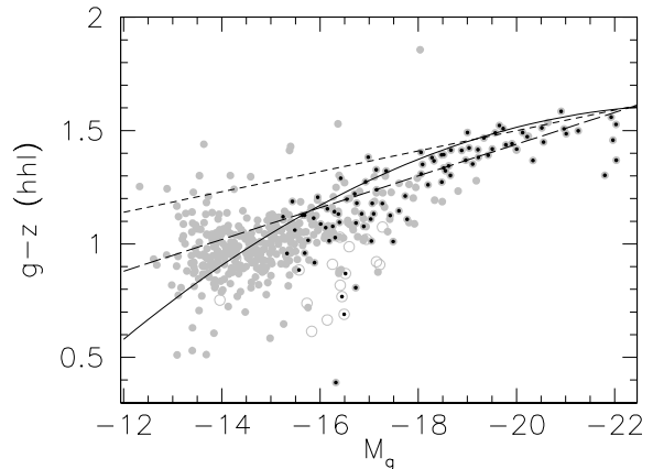
FIG. 3.— Comparison to the data of Ferrarese et al. (2006). Shown are all galaxies in our sample with gray symbols, again the blue-core dEs with open circles and the other galaxies with filled circles . Galaxies common to both samples are indicated by an additional black dot in the middle of the other symbol. The axes are changed in comparison to Fig. 1 and colors are measured in smaller apertures to most closely resemble their Fig. 123. The black lines indicate their fits to their data, the short dashed and long dashed line linear fits to a brighter ( M_g < -18 ) and fainter subsample ( M_g > -18 ), respectively. The solid line displays the parabola they fitted to the whole sample. There is a systematic offset of about 0.1 mag towards bluer colors of the color derived in our study in comparison to Ferrarese et al.
