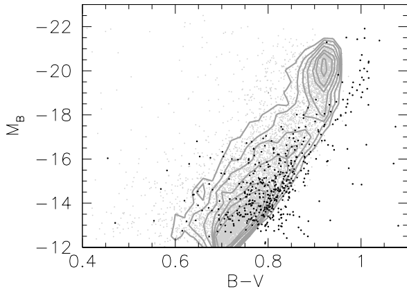
FIG. 2.— Color Magnitude Diagram, comparison to the semi-analytic model. Virgo cluster galaxies are shown with black symbols and model galaxies from the Numerical Galaxy Catalog (Nagashima et al. 2005) as gray dots (we selected galaxies with B/T > 0.6 and with higher effective surface brightness than 25.5 \text{ mag arcsec}^{-2} ). Contours were calculated using model galaxy abundances in bins of 0.5 mag in brightness and 0.02 mag in color. The contour levels, relative to the lowest level, are 2, 3.4, 5, 7.5, 10, and 15.
